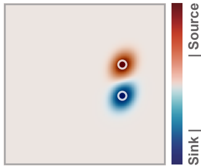
Simulated CSD + CMs
